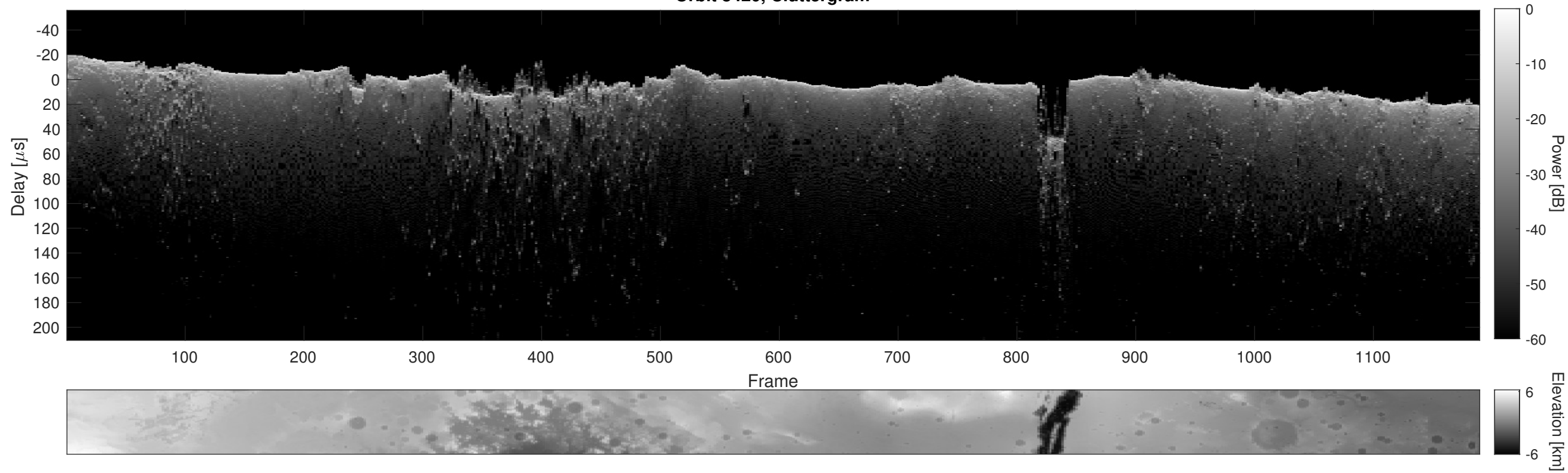
Orbit 8420, Cluttergram
