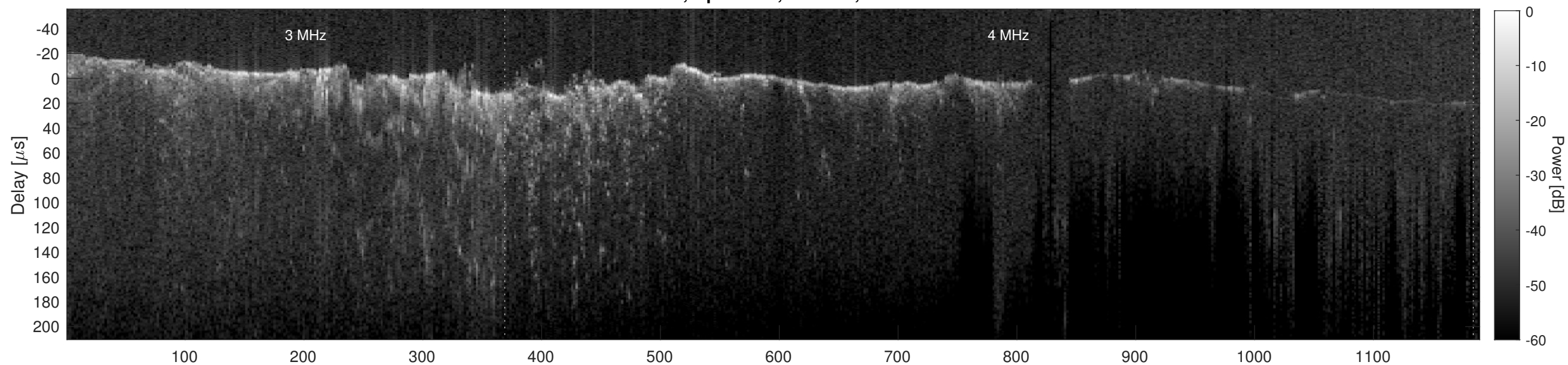
Orbit 8420, Cluttergram
