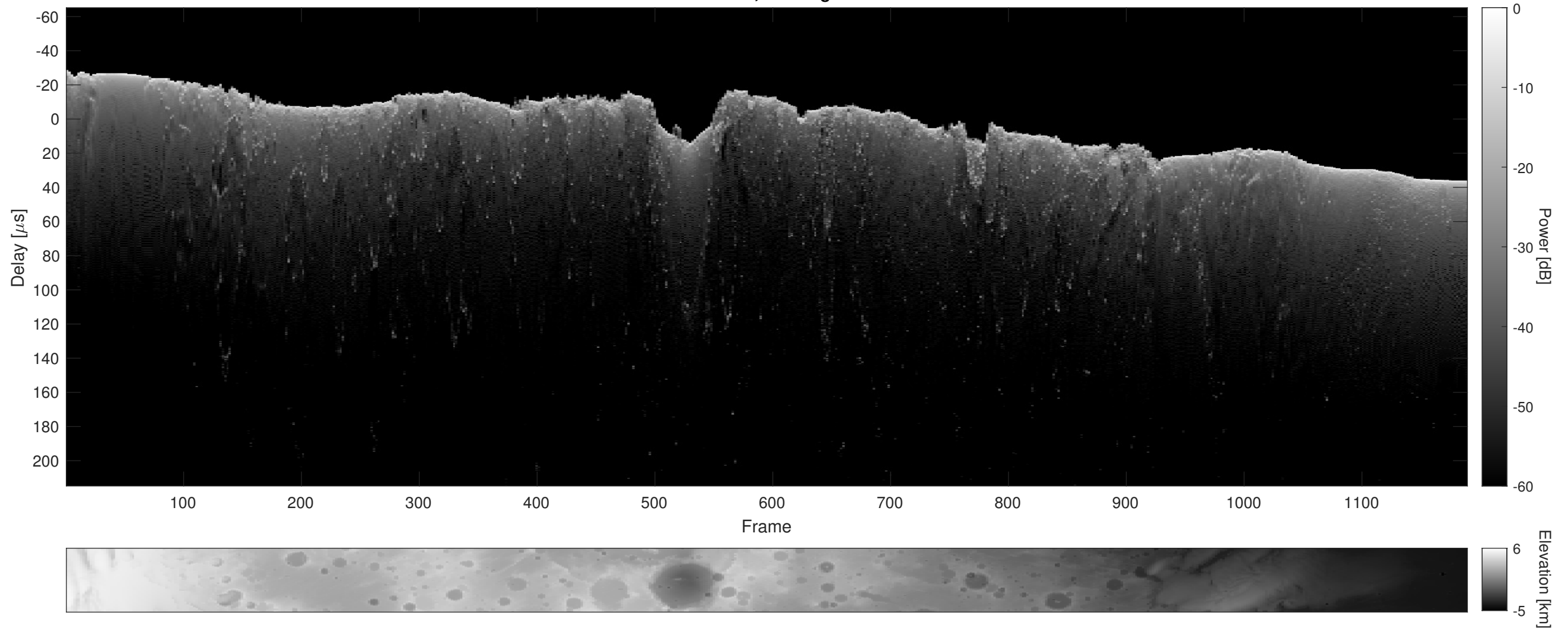
Orbit 8421, Cluttergram
