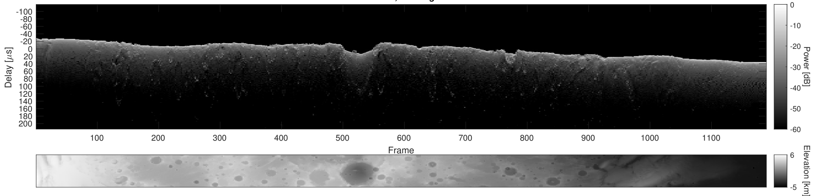
Orbit 8421, Cluttergram
