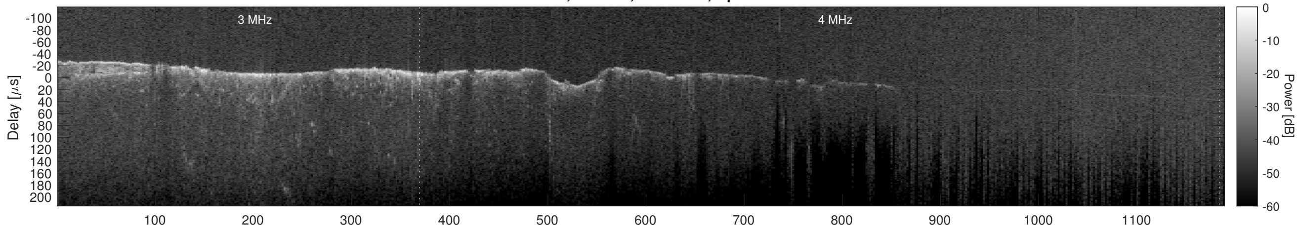
Orbit 8421, Cluttergram
