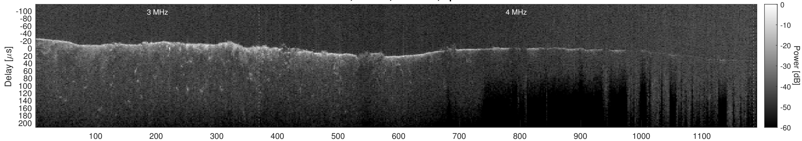
Orbit 8422, Cluttergram
