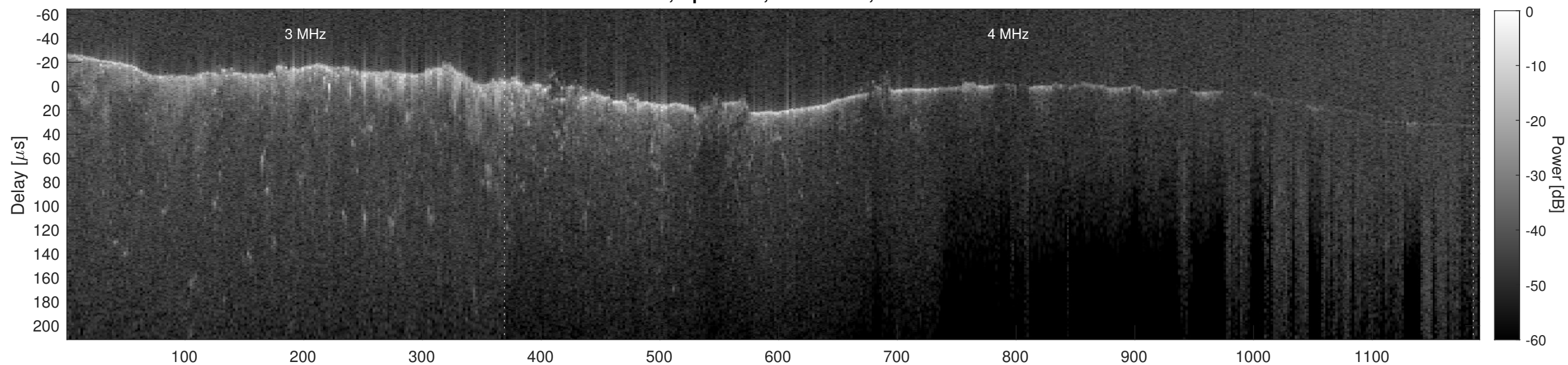
Orbit 8422, Cluttergram
