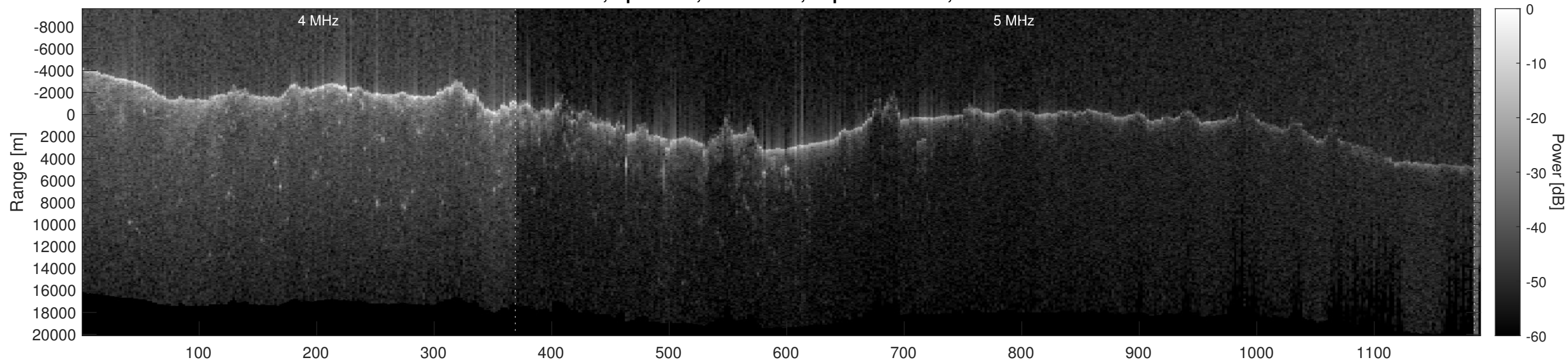
Orbit 8422, Optimized, No Window, Depth-Corrected, Channel 2
