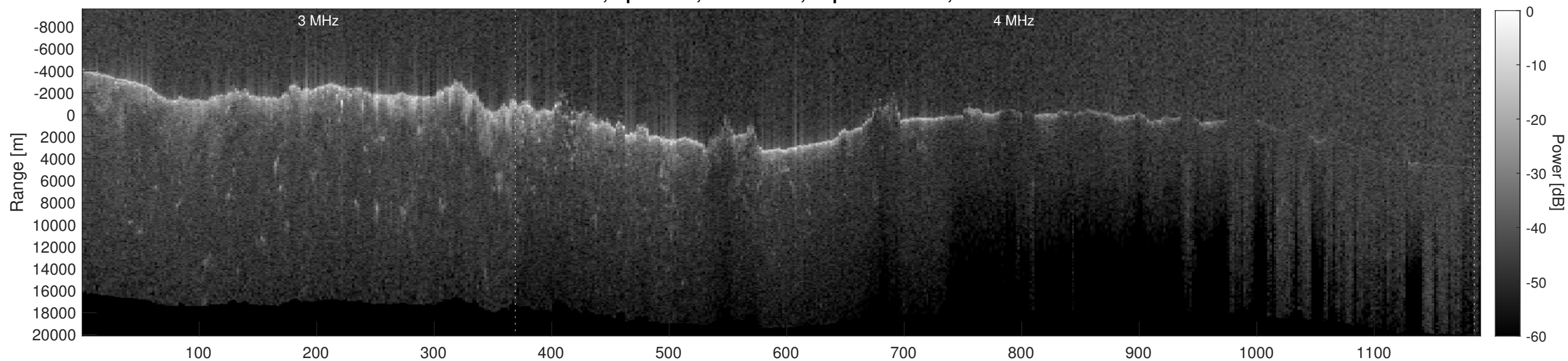
Orbit 8422, Depth-Corrected Cluttergram
