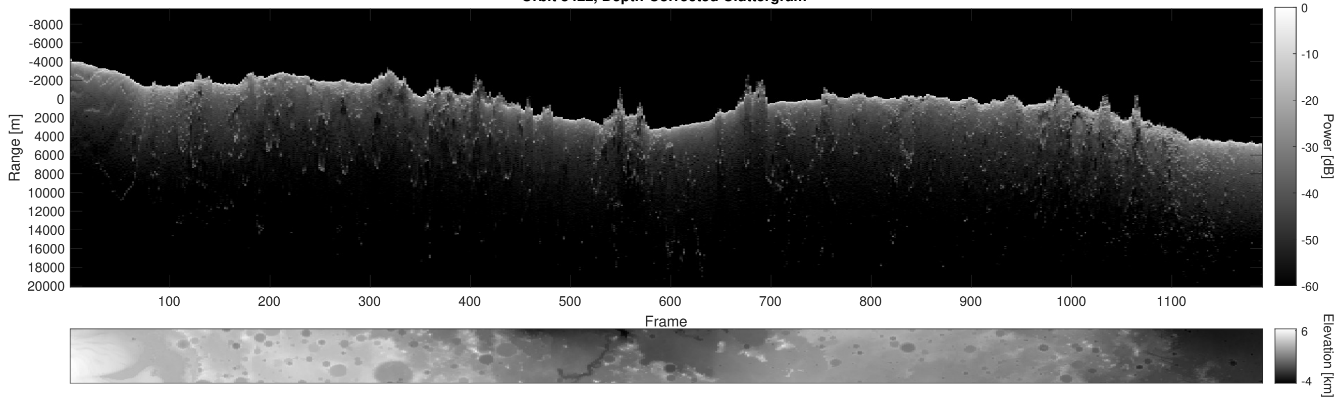
Orbit 8422, Depth-Corrected Cluttergram
