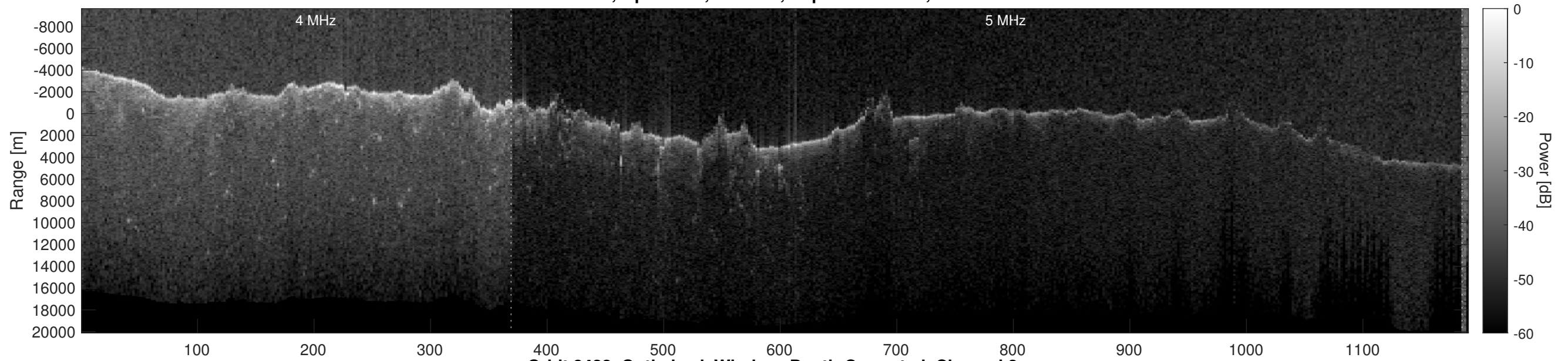
Orbit 8422, Optimized, Window, Depth-Corrected, Channel 2
