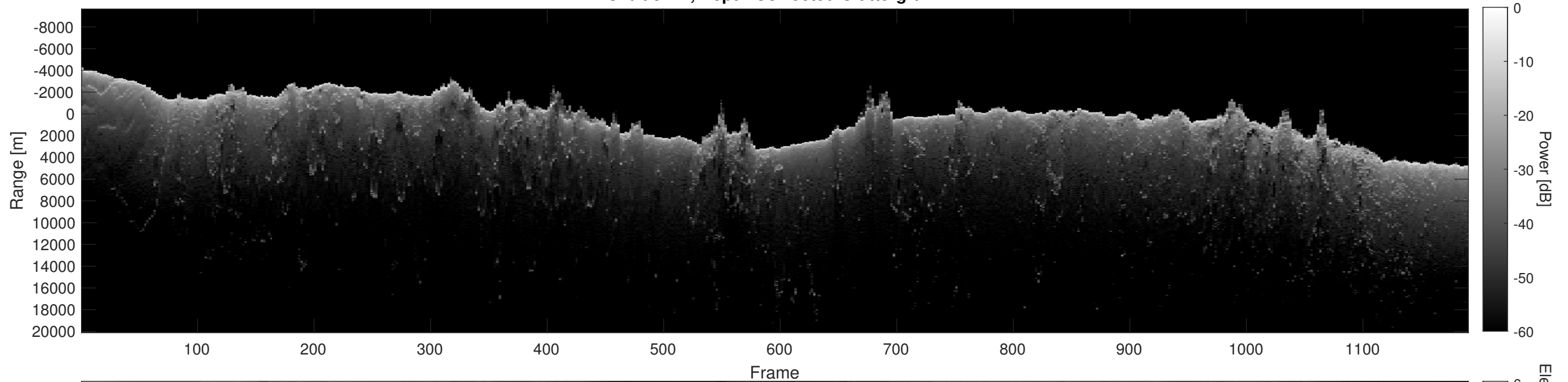
Orbit 8422, Depth-Corrected Cluttergram
