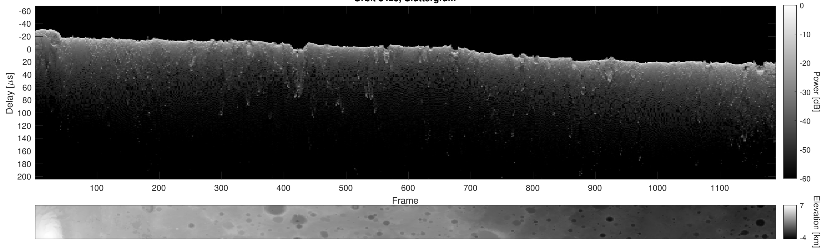
Orbit 8423, Cluttergram
