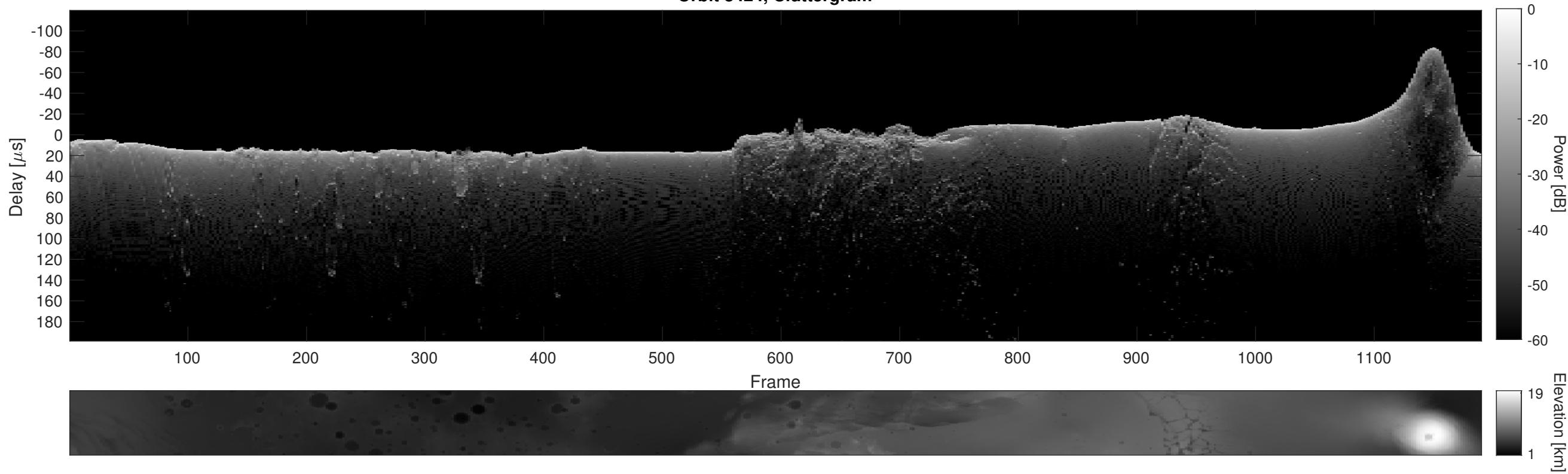
Orbit 8424, Cluttergram
