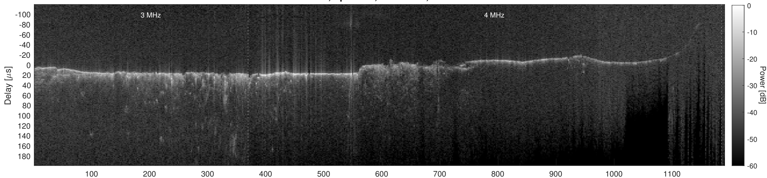
Orbit 8424, Cluttergram
