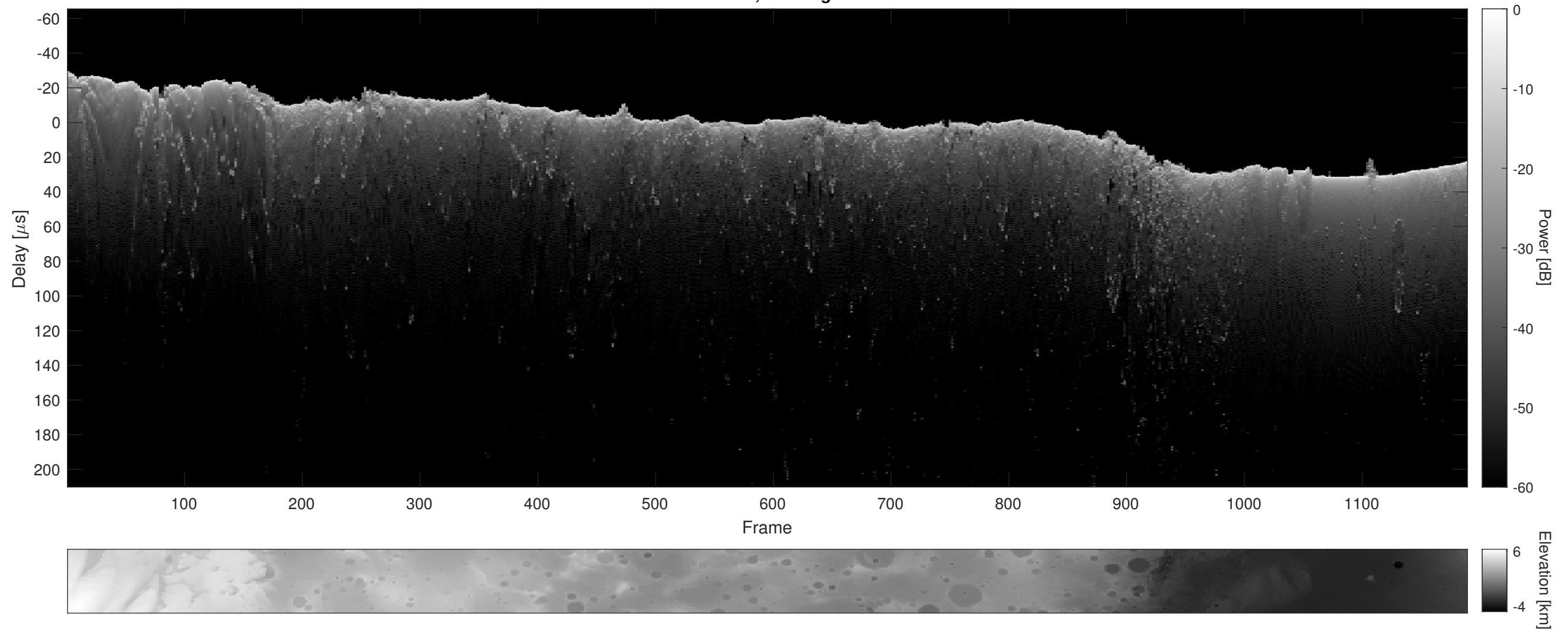
Orbit 8425, Cluttergram
