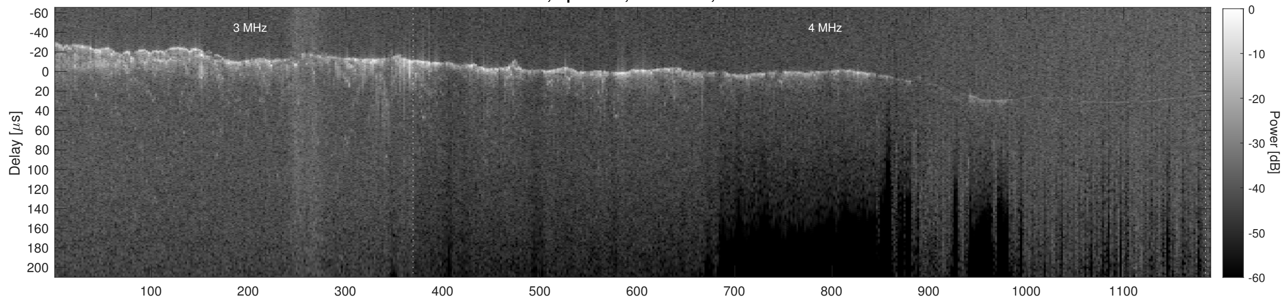
Orbit 8425, Cluttergram
