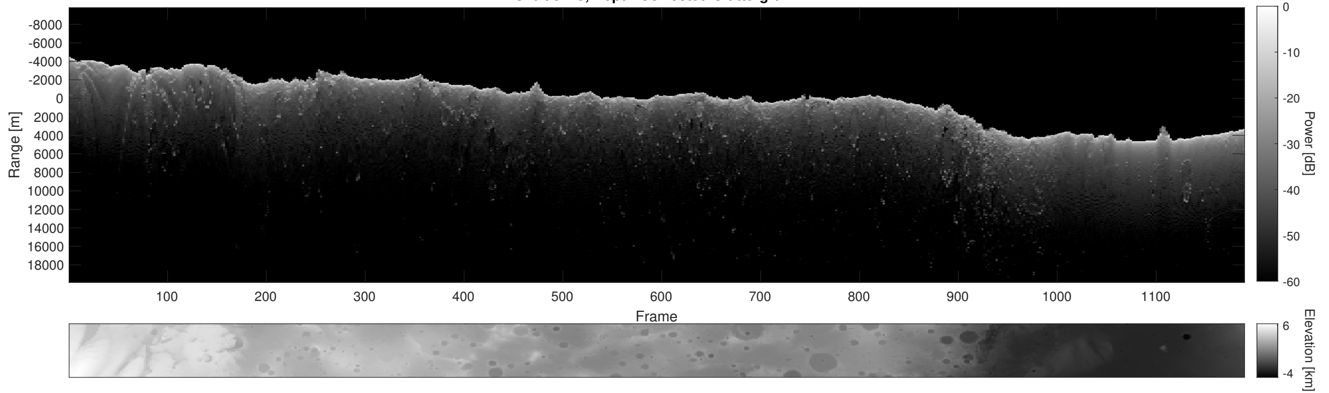
Orbit 8425, Depth-Corrected Cluttergram
