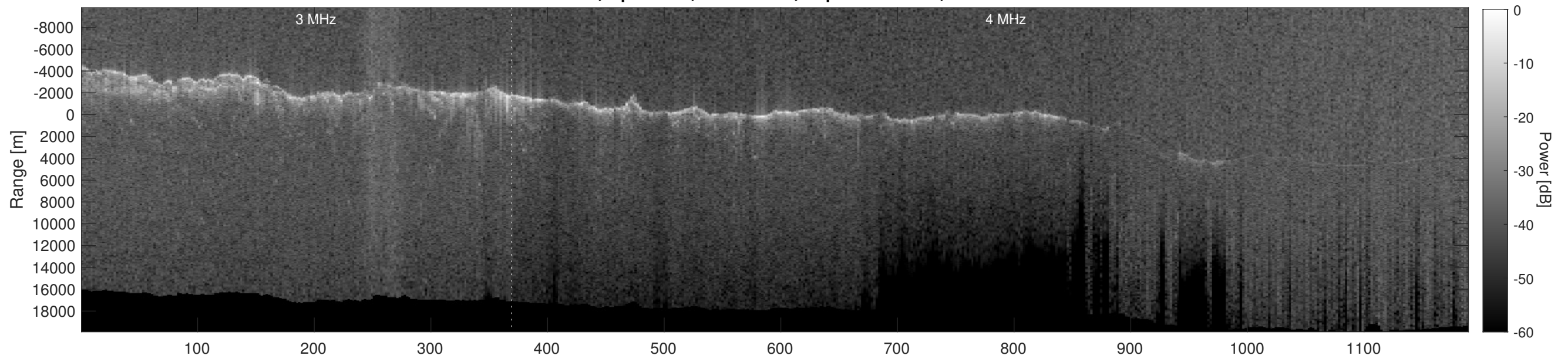
Orbit 8425, Depth-Corrected Cluttergram
