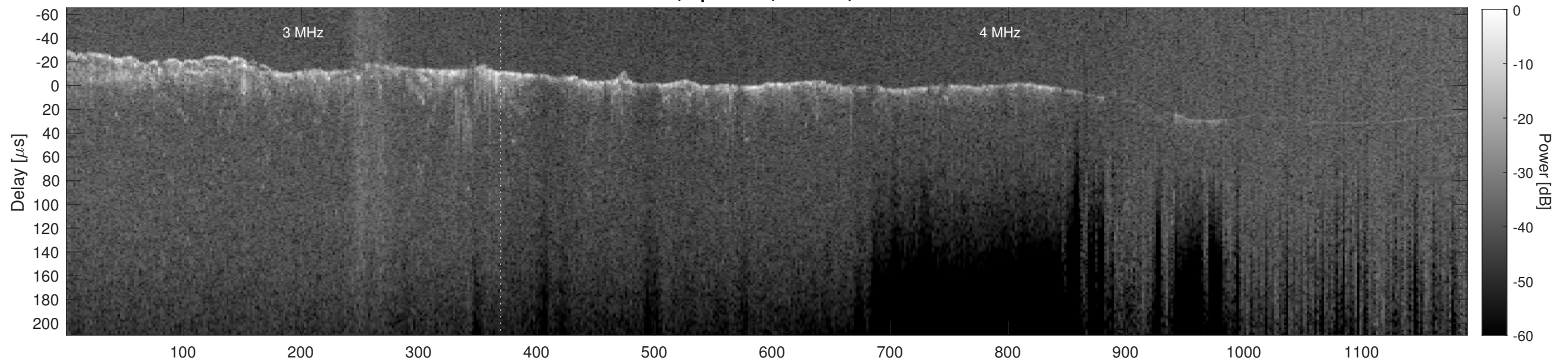
Orbit 8425, Cluttergram
