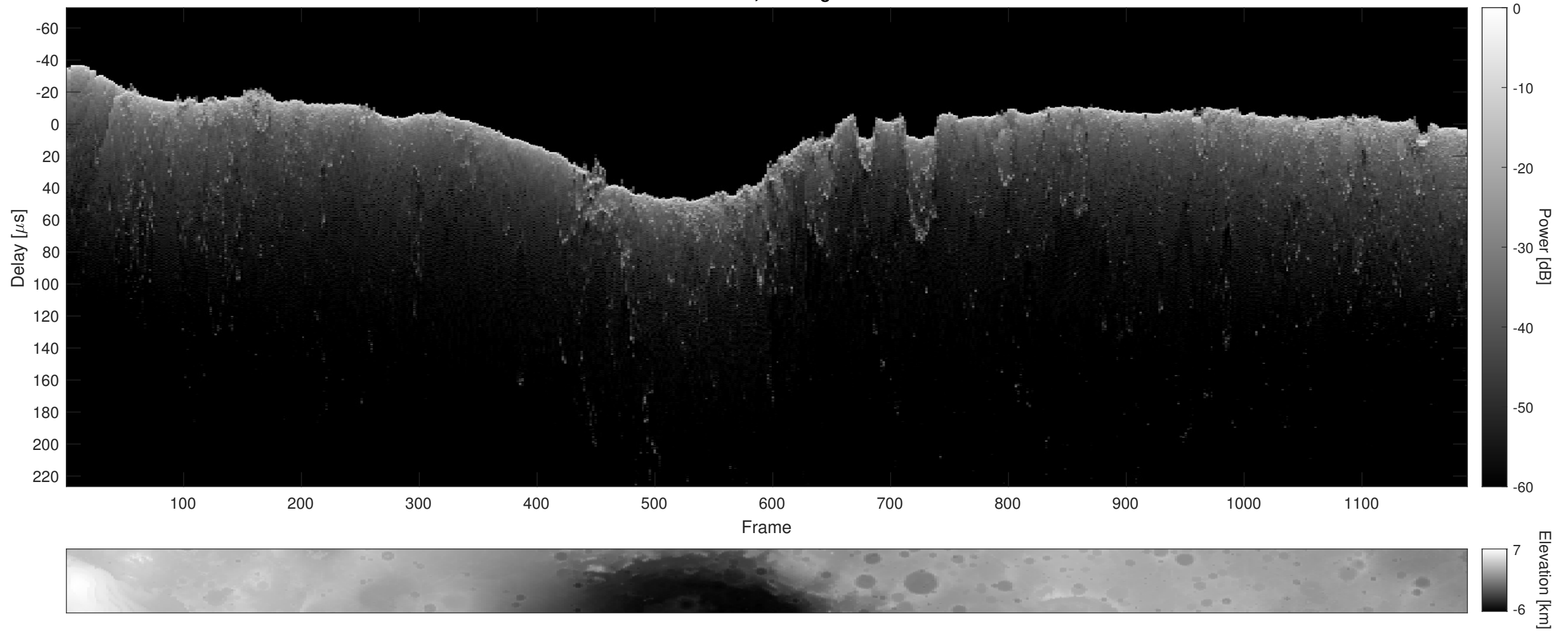
Orbit 8426, Cluttergram
