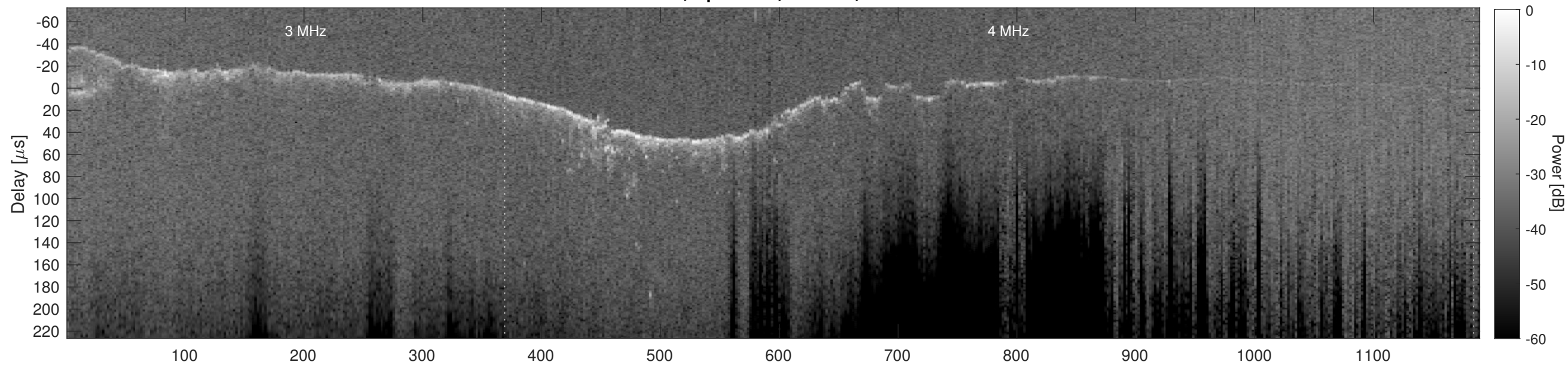
Orbit 8426, Cluttergram
