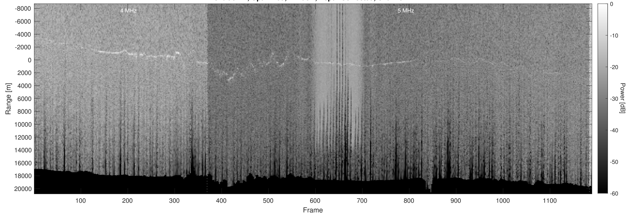
Orbit 8427, Optimized, Window, Depth-Corrected, Channel 2
