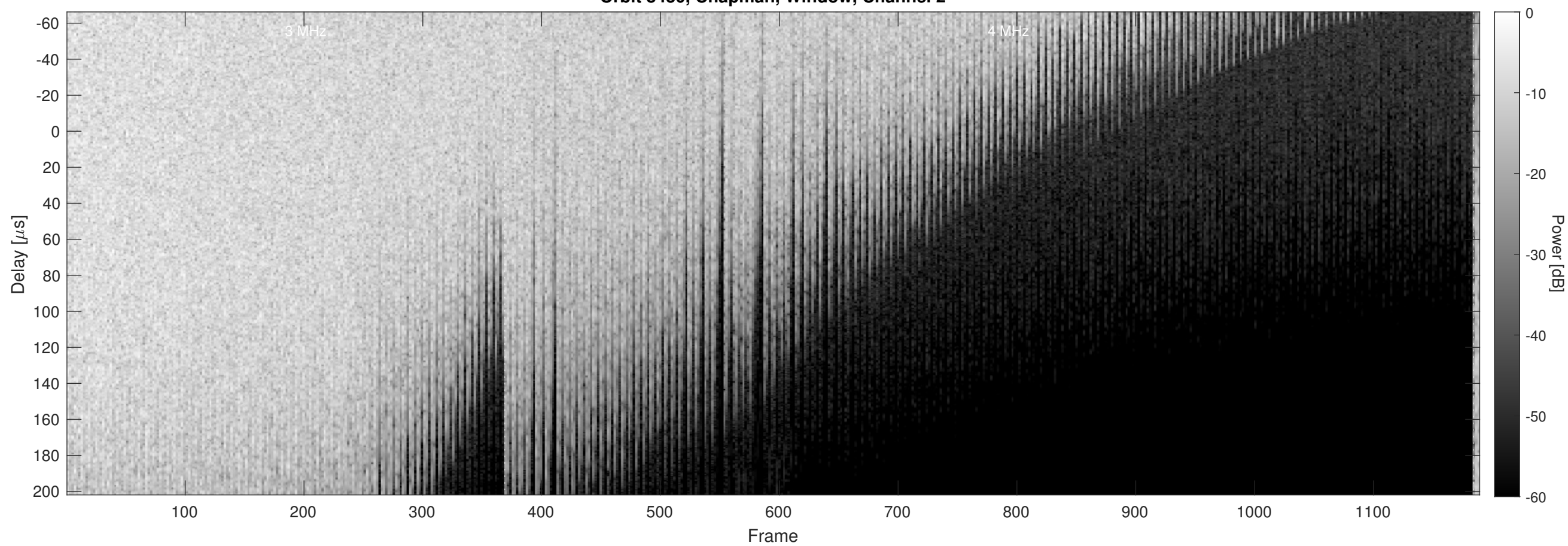
Orbit 8430, Chapman, Window, Channel 2
