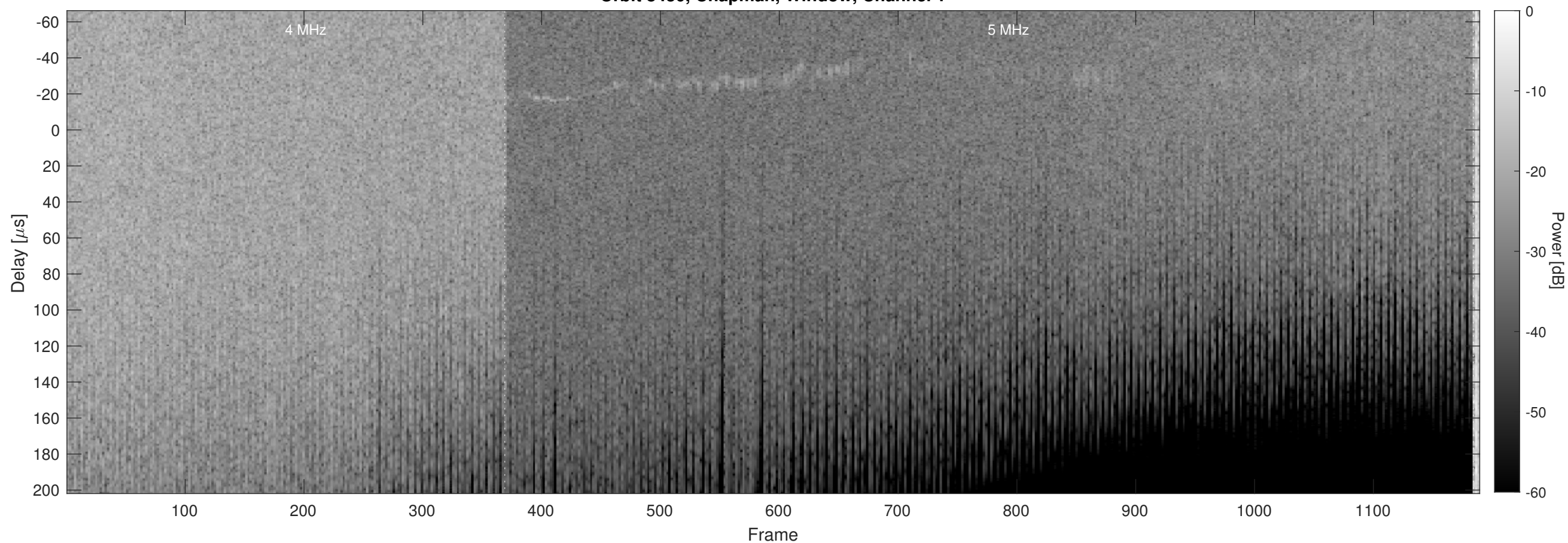
Orbit 8430, Chapman, Window, Channel 2
