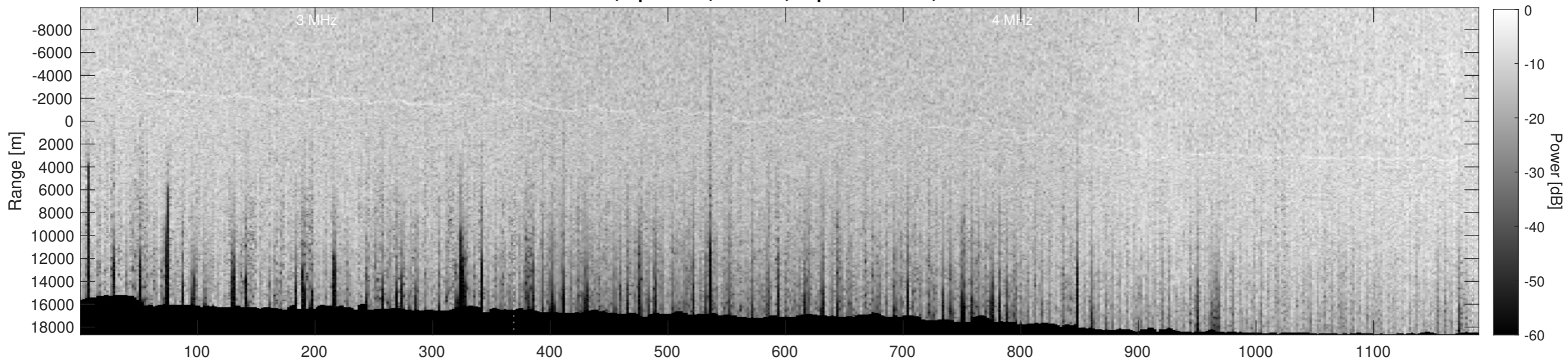
Orbit 8430, Depth-Corrected Cluttergram
