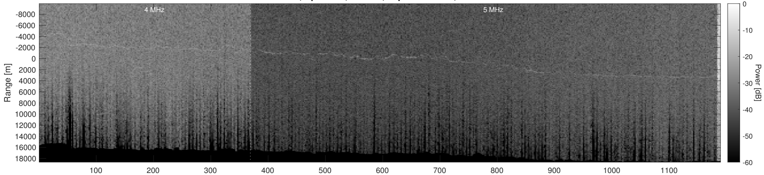
Orbit 8430, Optimized, Window, Depth-Corrected, Channel 2
