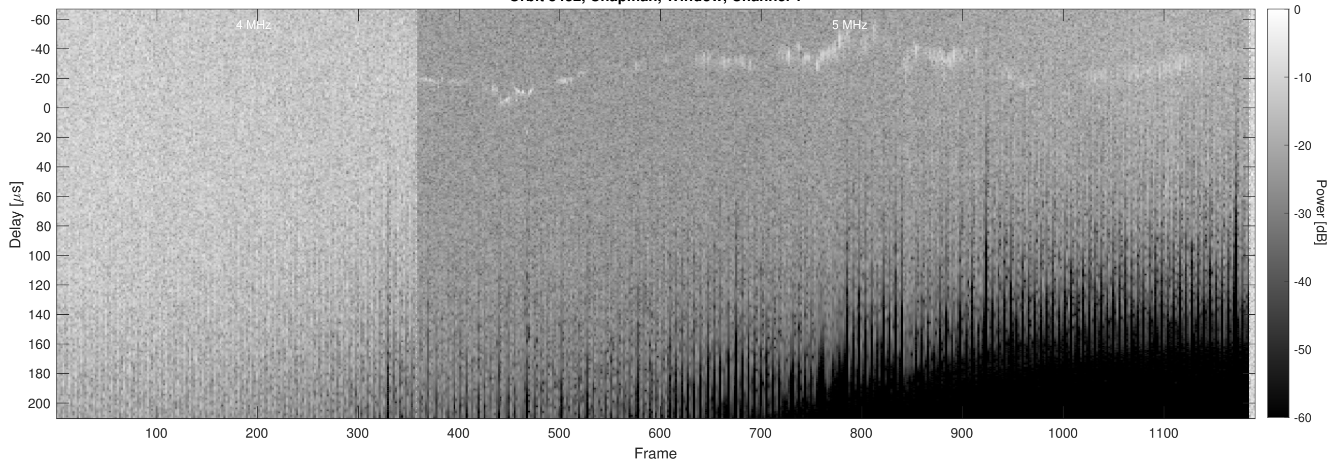
Orbit 8432, Chapman, Window, Channel 2
