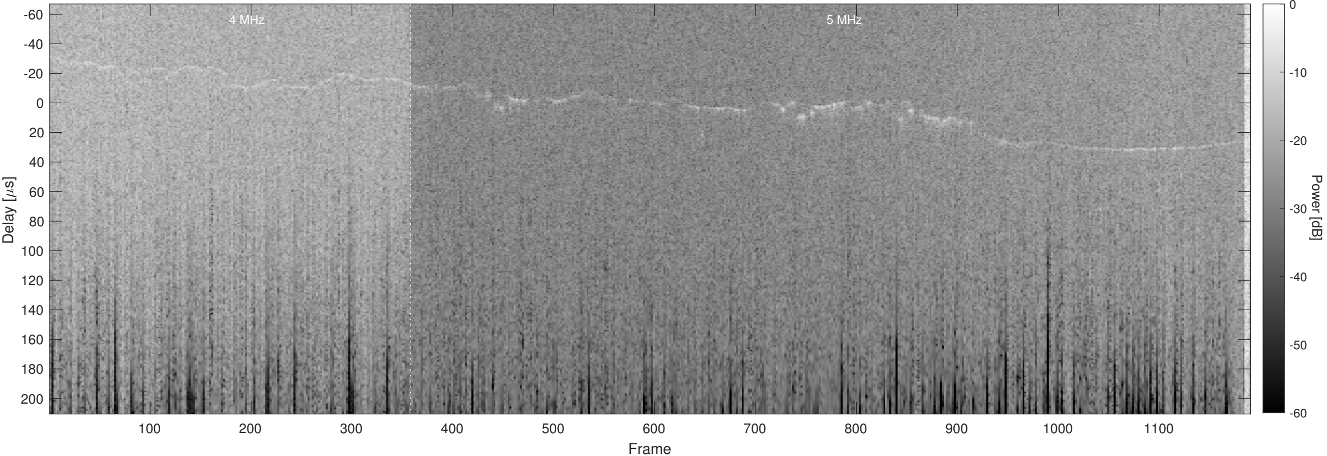
Orbit 8432, Optimized, No Window, Channel 2
