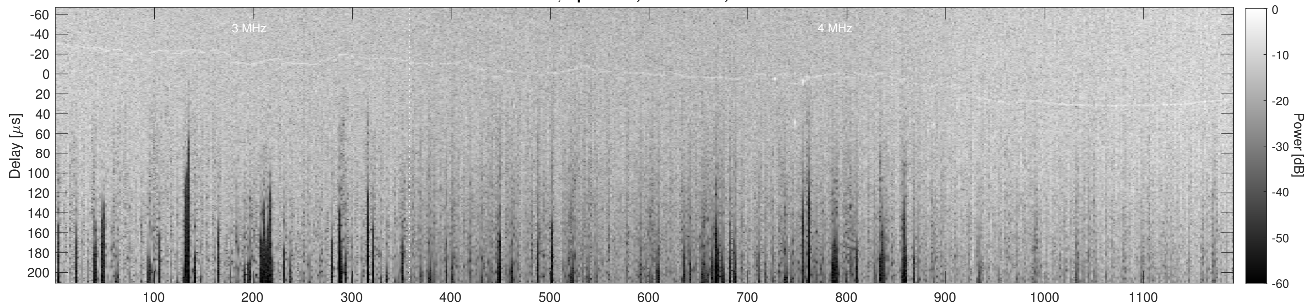
Orbit 8432, Cluttergram
