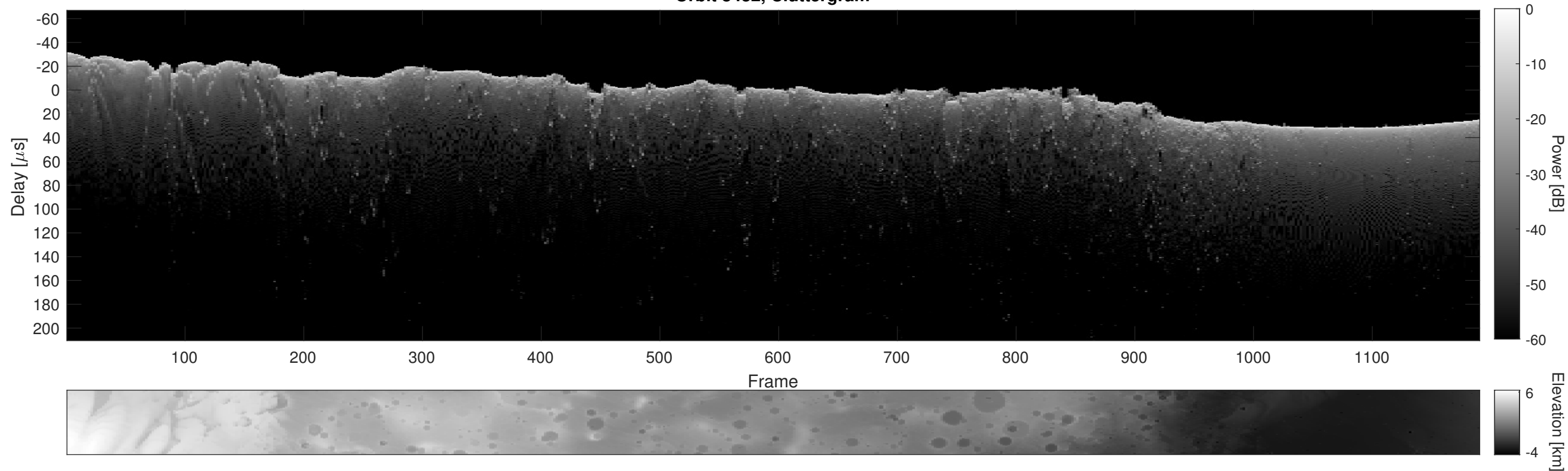
Orbit 8432, Cluttergram
