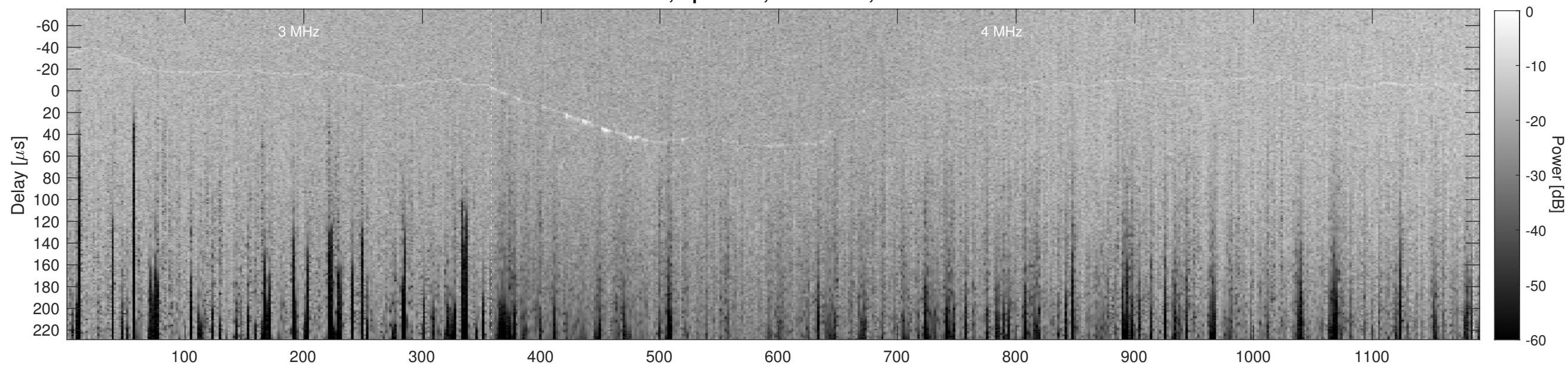
Orbit 8433, Cluttergram
