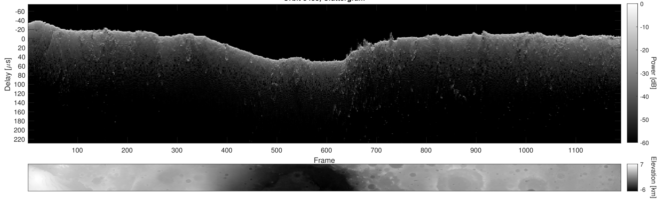
Orbit 8433, Cluttergram
