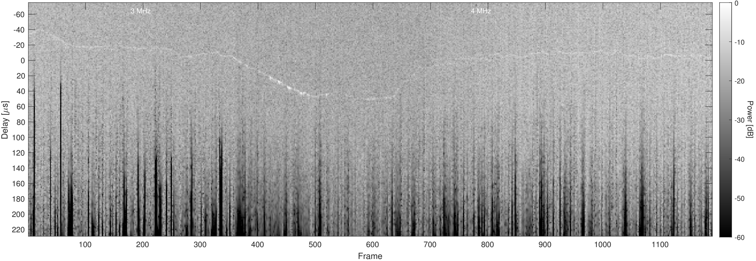
Orbit 8433, Optimized, Window, Channel 2
