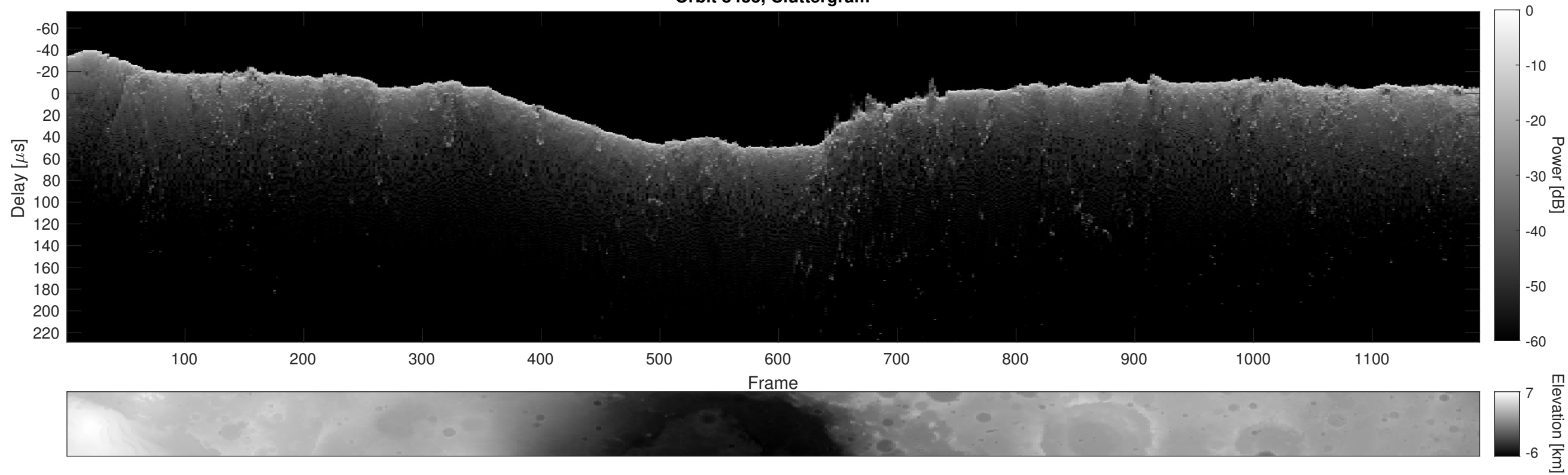
Orbit 8433, Cluttergram
