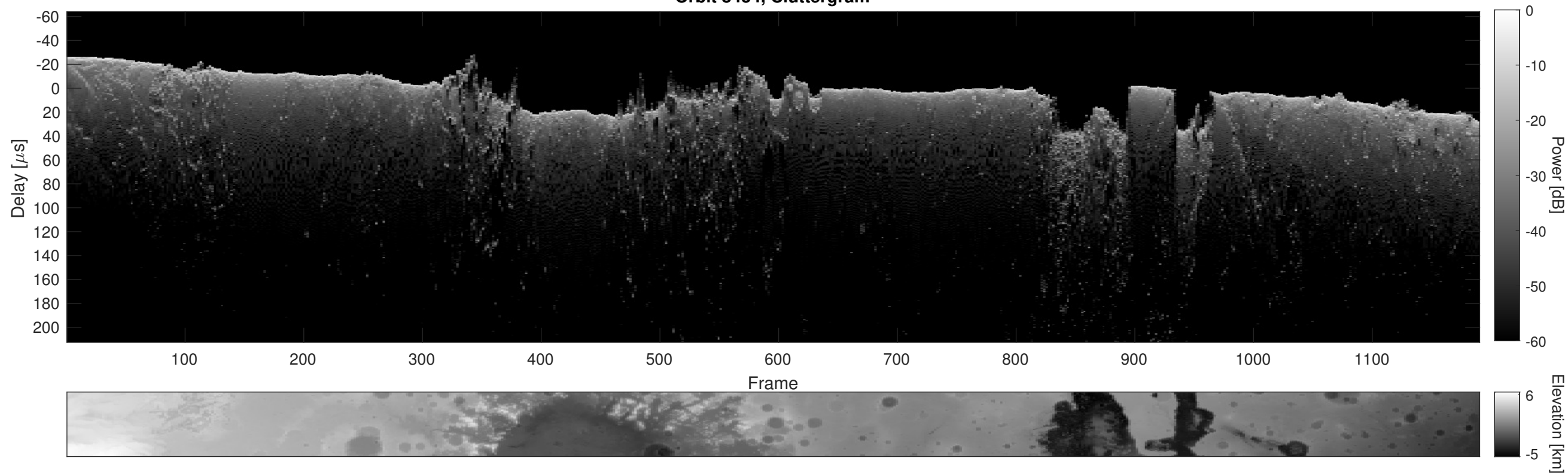
Orbit 8434, Cluttergram
