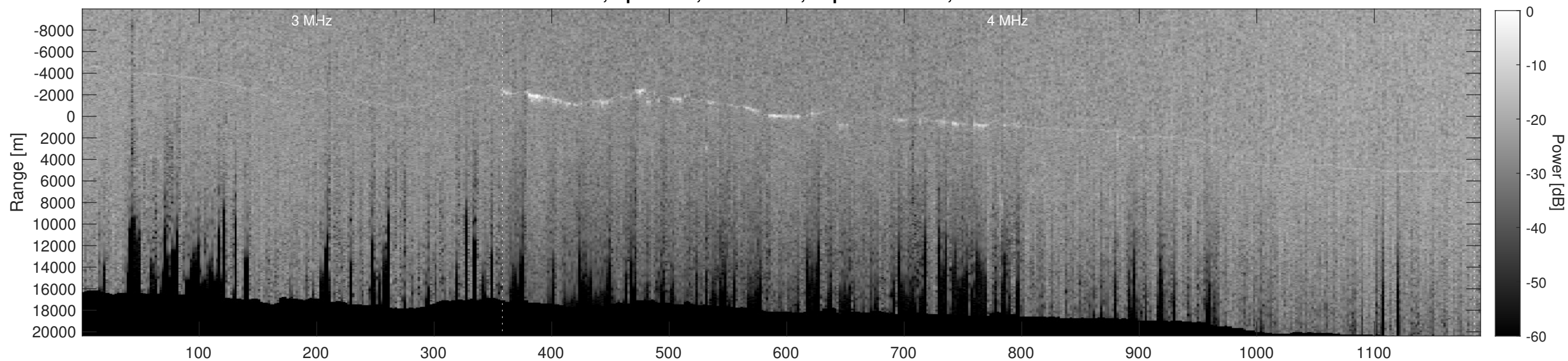
Orbit 8435, Depth-Corrected Cluttergram
