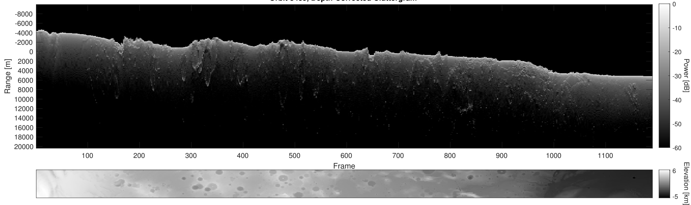
Orbit 8435, Depth-Corrected Cluttergram
