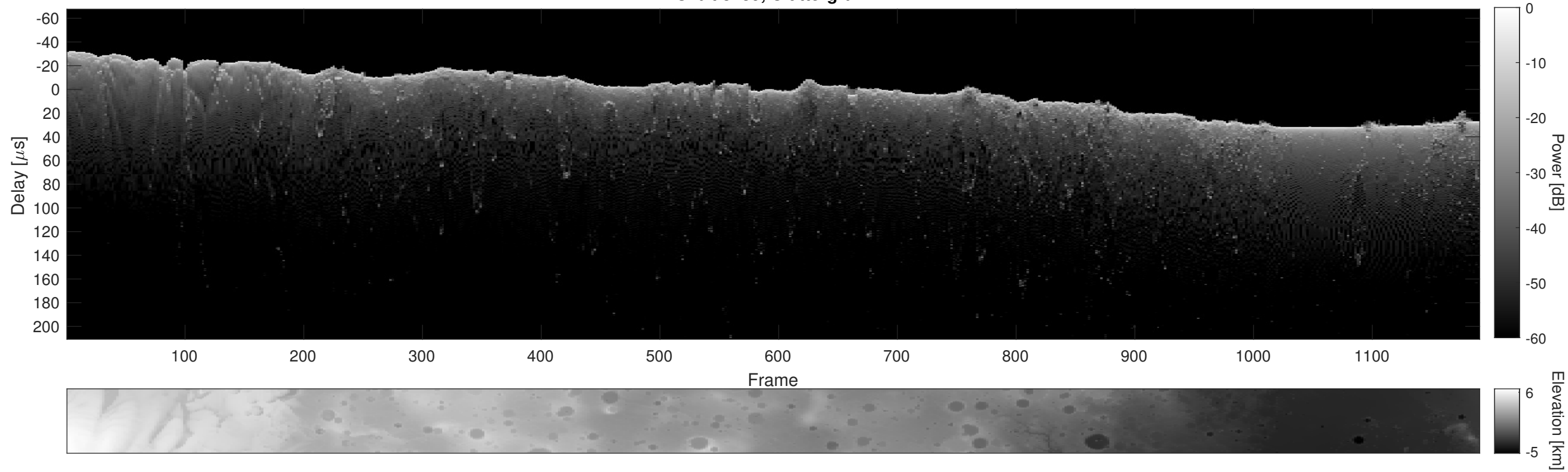
Orbit 8439, Cluttergram
