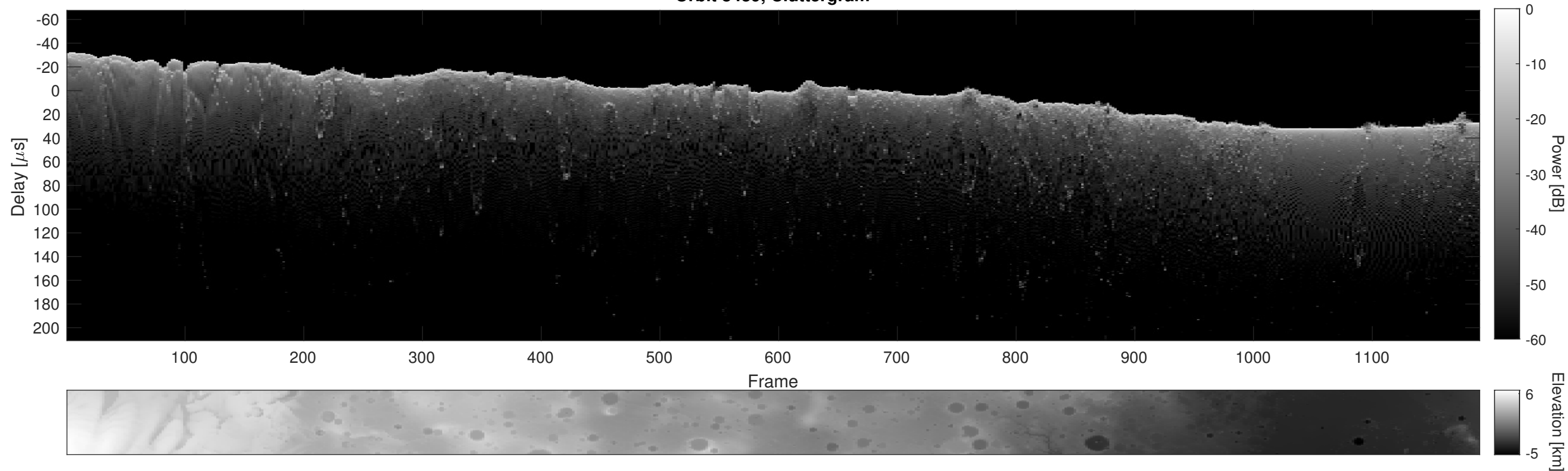
Orbit 8439, Cluttergram
