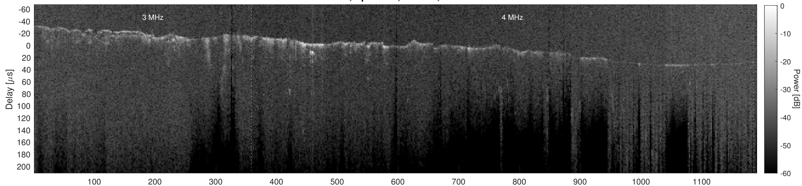
Orbit 8439, Cluttergram
