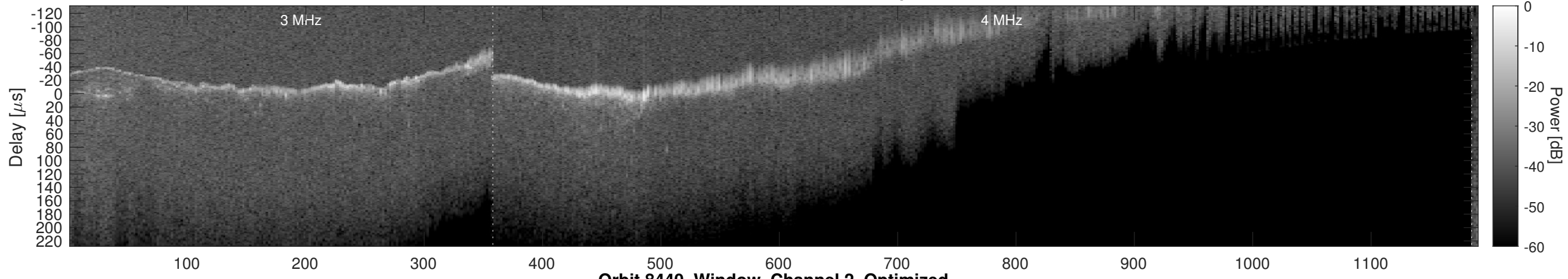
Orbit 8440, Window, Channel 2, Optimized
