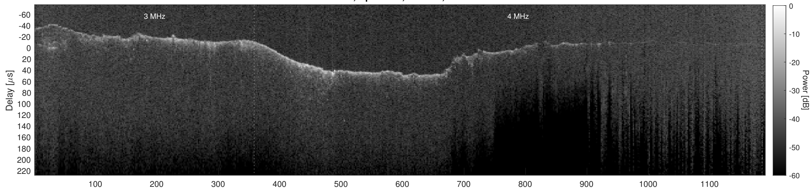
Orbit 8440, Cluttergram
