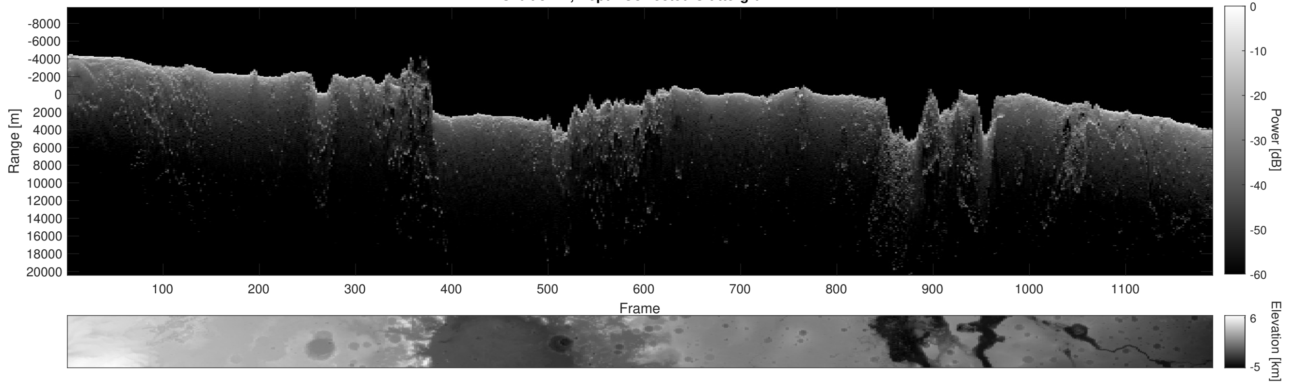
Orbit 8441, Depth-Corrected Cluttergram
