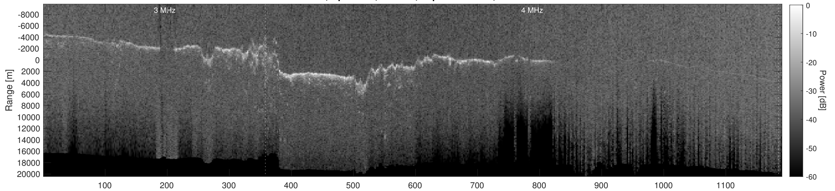
Orbit 8441, Depth-Corrected Cluttergram
