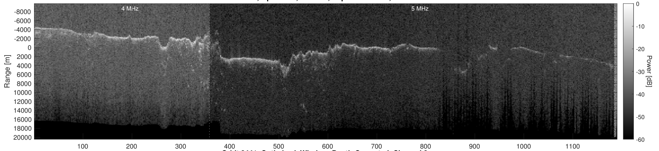
Orbit 8441, Optimized, Window, Depth-Corrected, Channel 2
