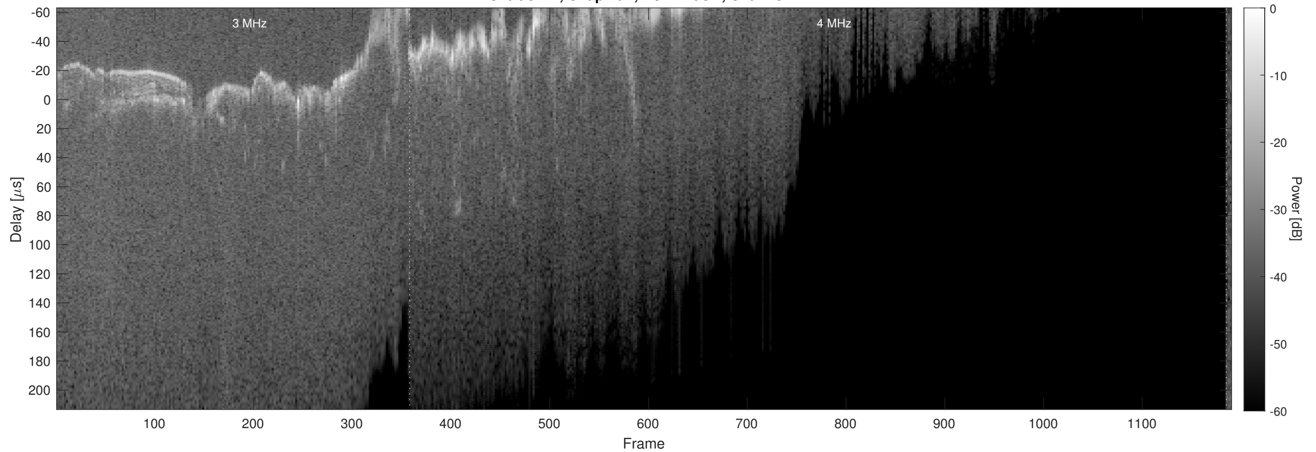
Orbit 8442, Chapman, No Window, Channel 2
