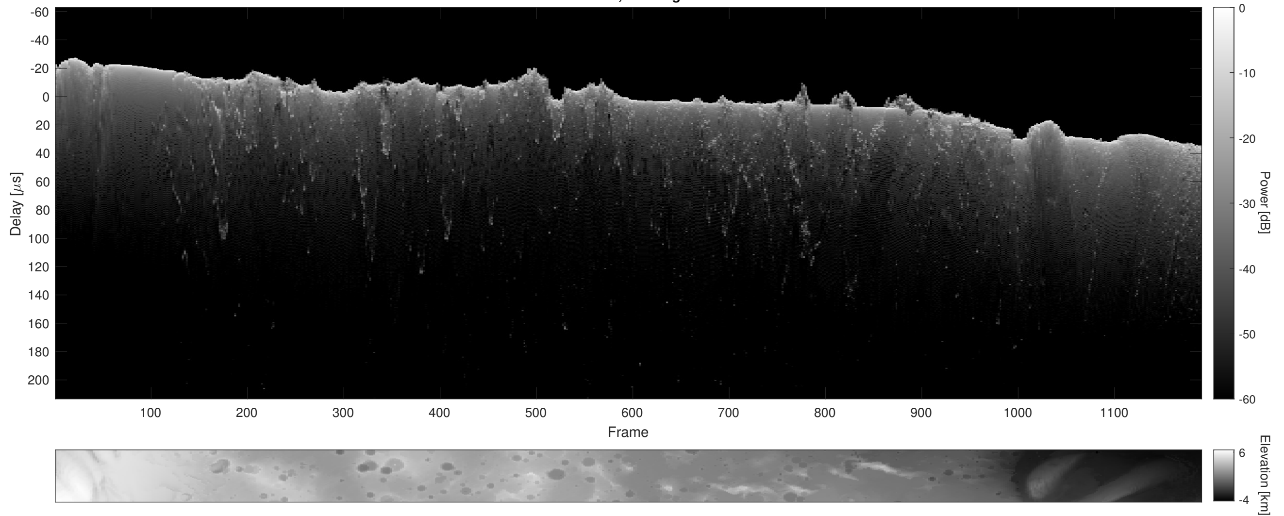
Orbit 8442, Cluttergram
