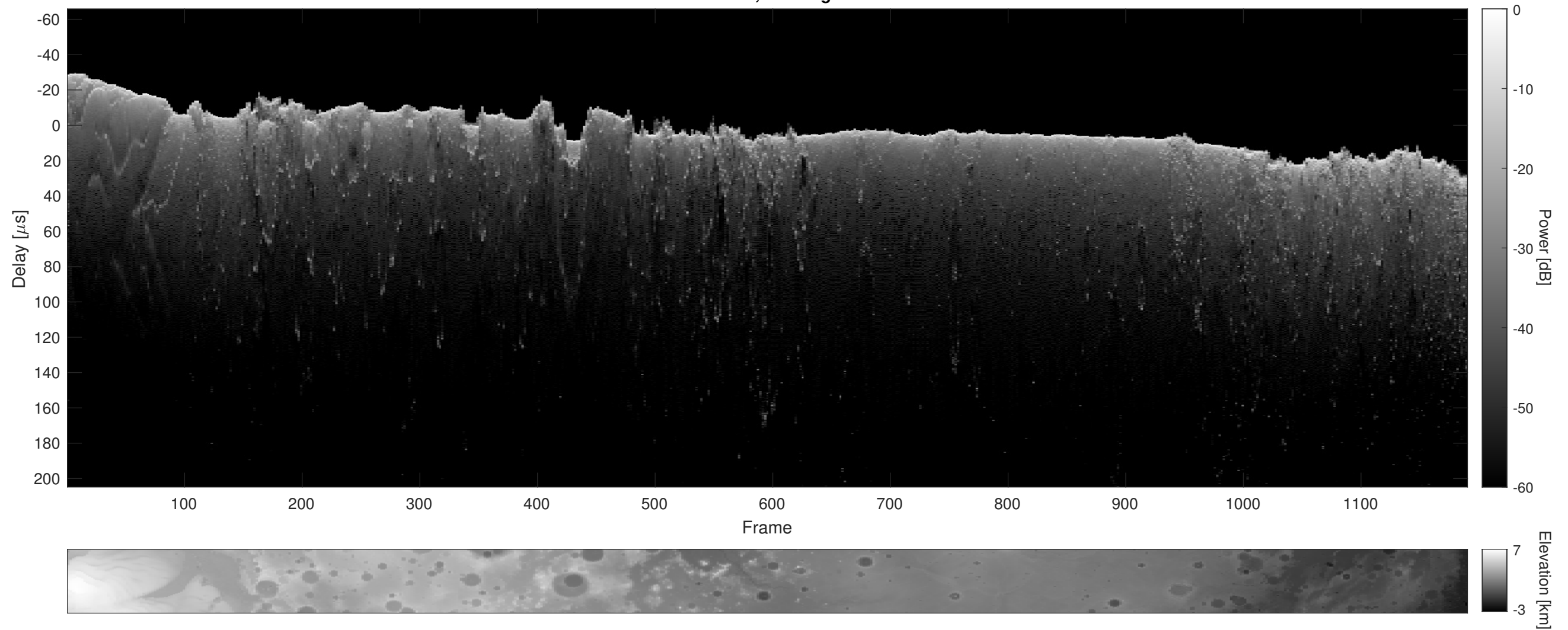
Orbit 8443, Cluttergram
