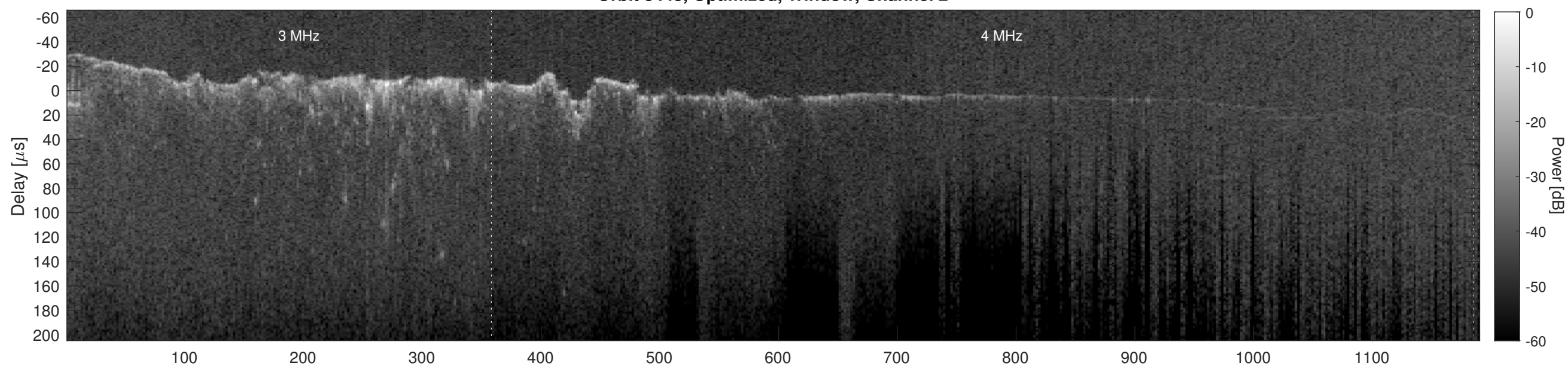
Orbit 8443, Cluttergram
