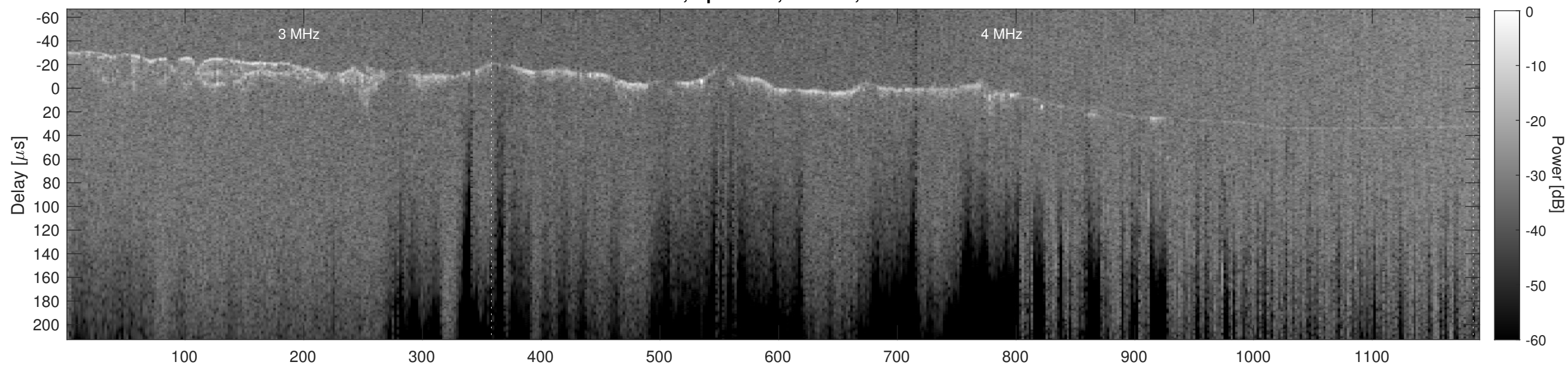
Orbit 8446, Cluttergram
