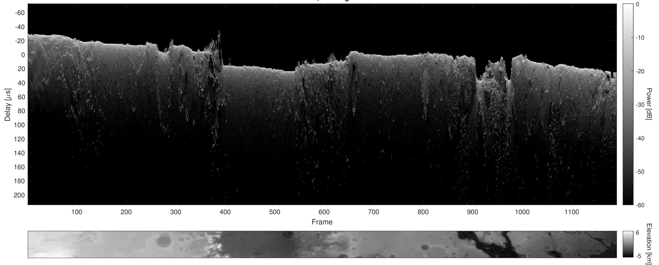
Orbit 8448, Cluttergram
