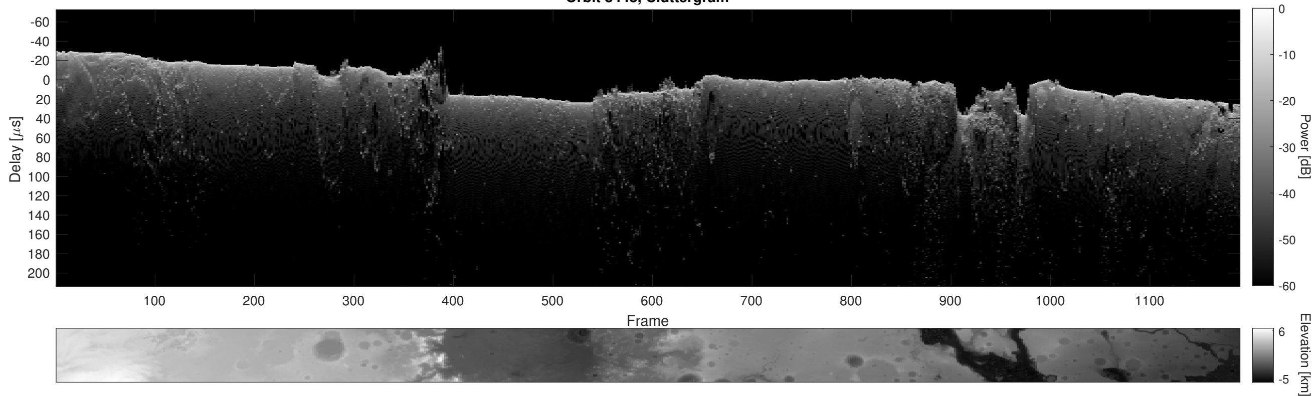
Orbit 8448, Cluttergram
