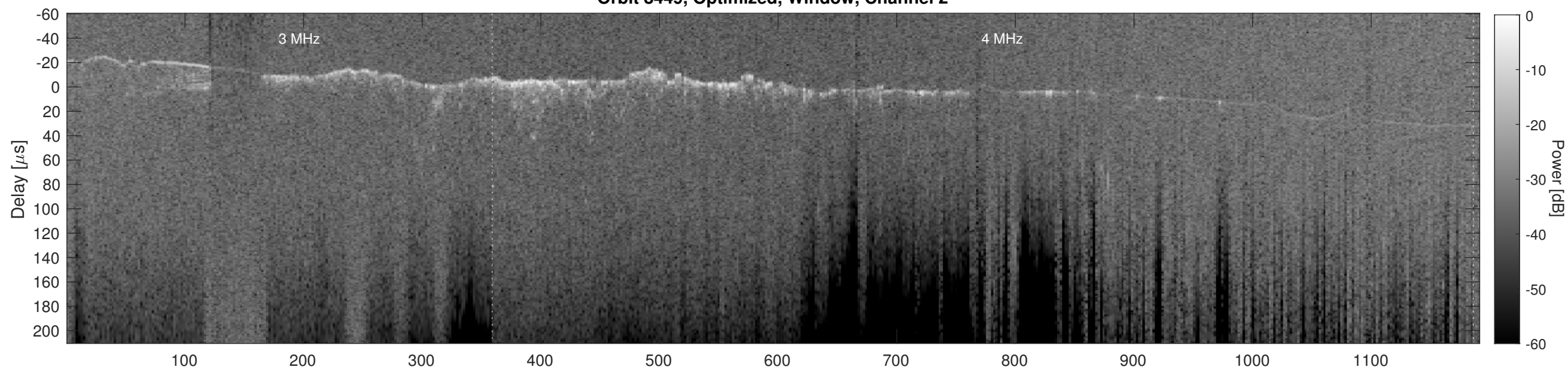
Orbit 8449, Cluttergram
