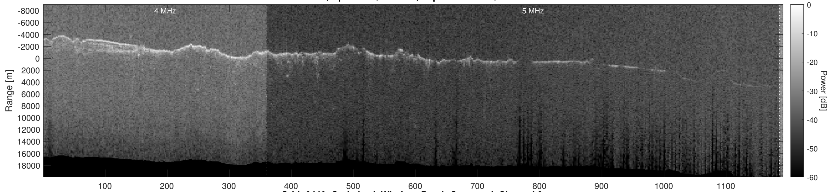
Orbit 8449, Optimized, Window, Depth-Corrected, Channel 2
