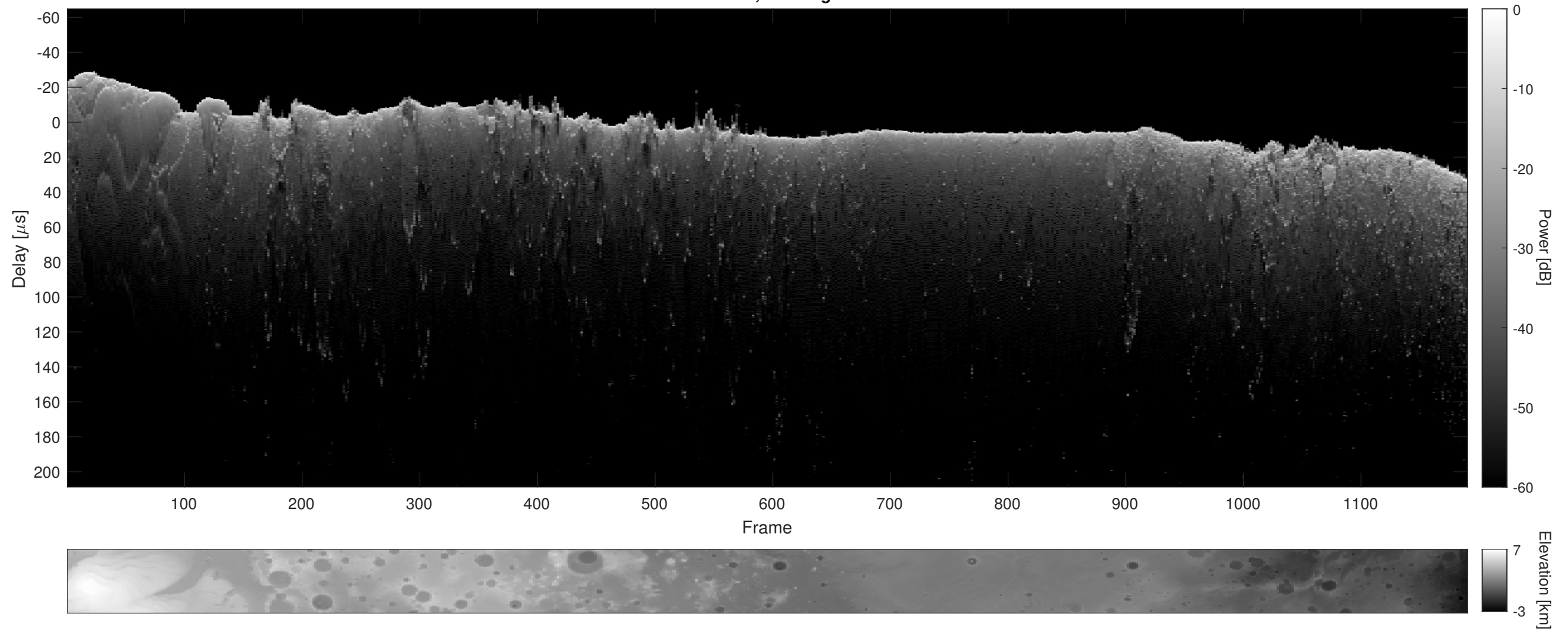
Orbit 8450, Cluttergram
