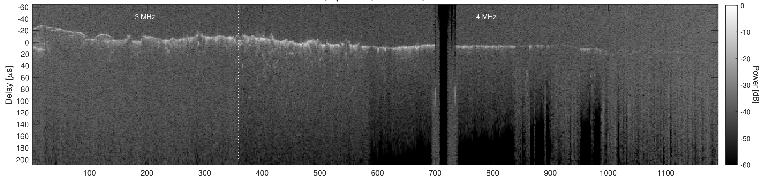
Orbit 8450, Cluttergram
