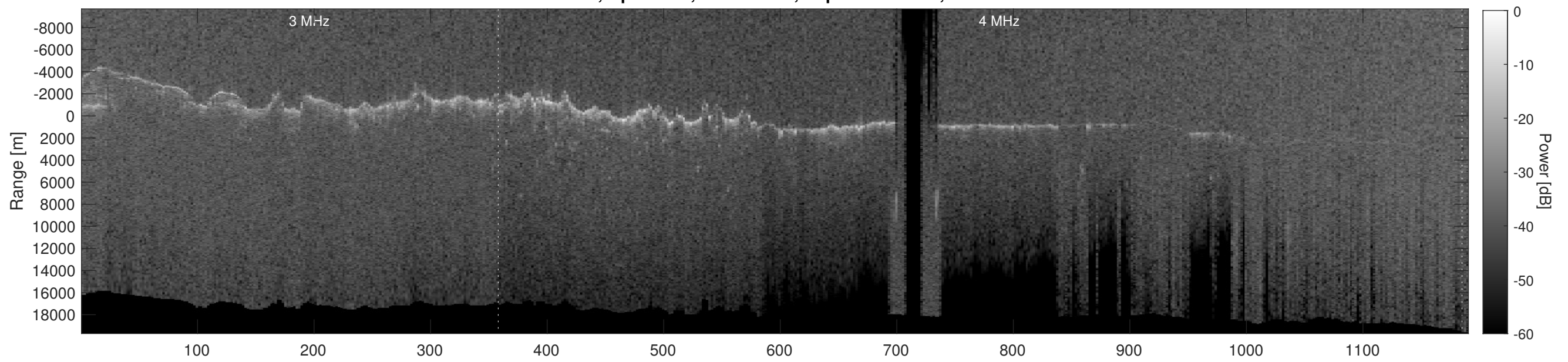
Orbit 8450, Depth-Corrected Cluttergram
