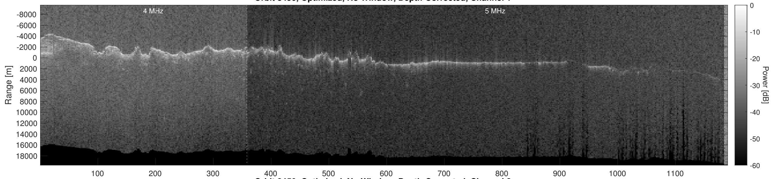
Orbit 8450, Optimized, No Window, Depth-Corrected, Channel 2
