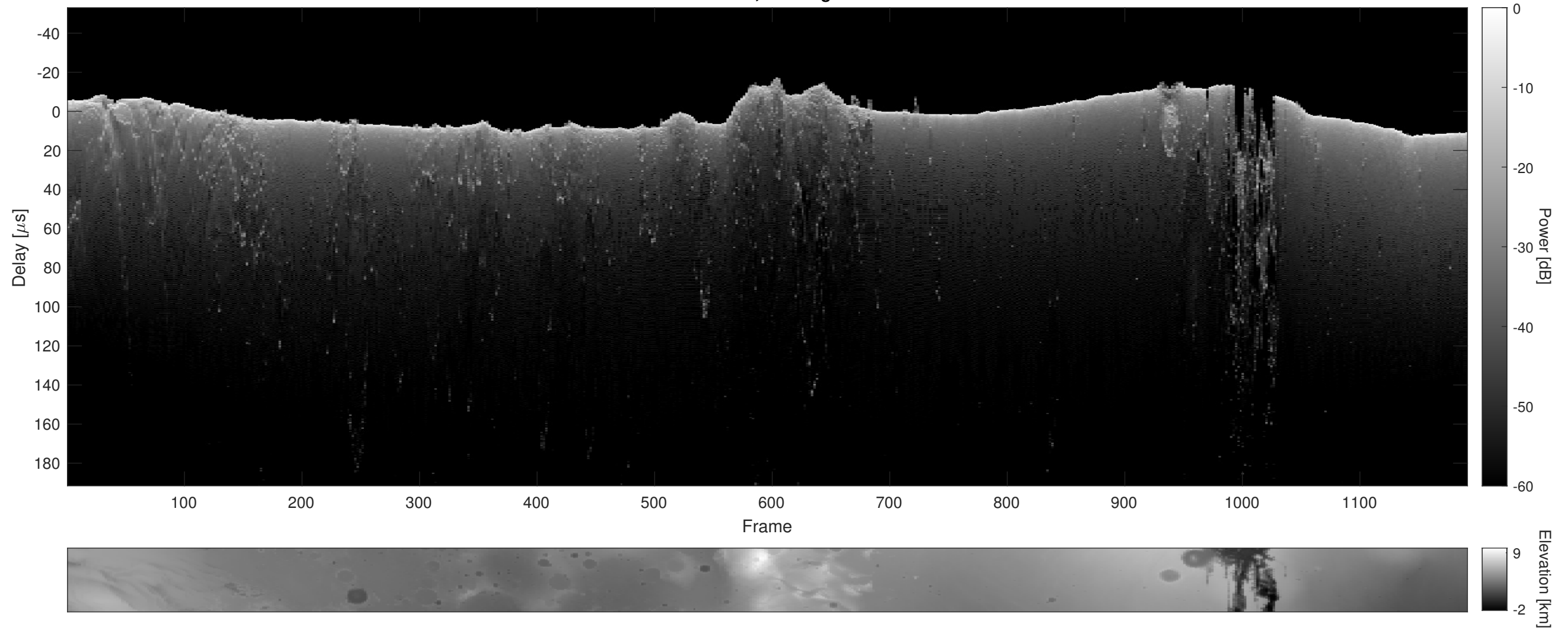
Orbit 8452, Cluttergram
