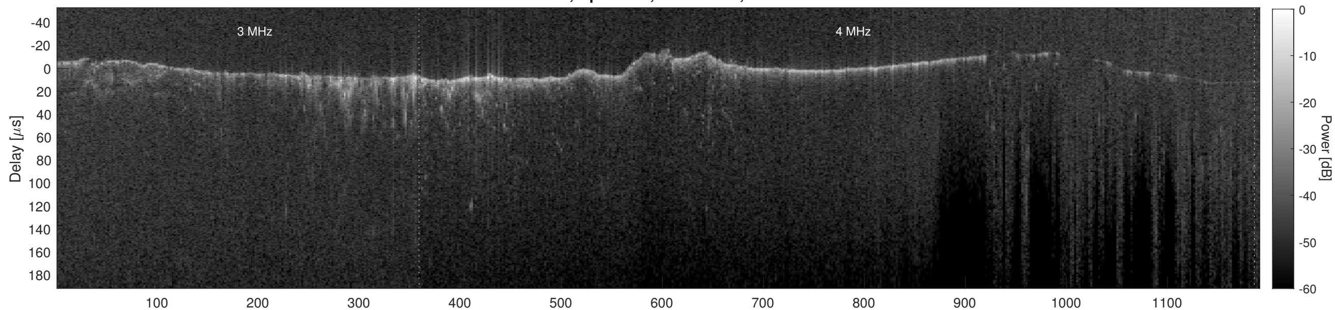
Orbit 8452, Cluttergram
