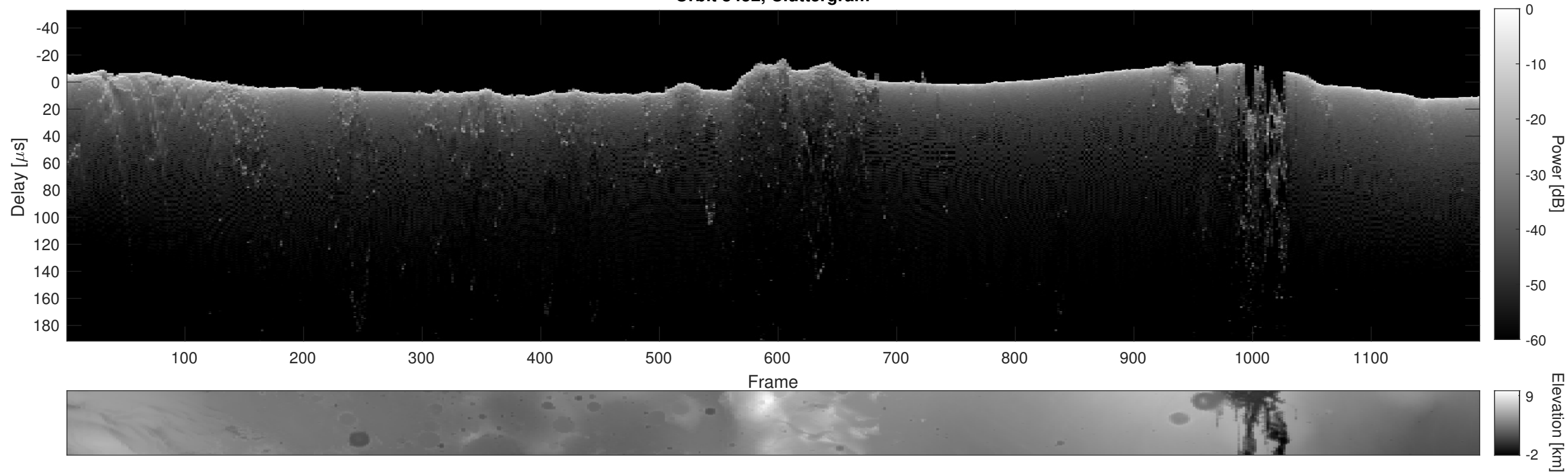
Orbit 8452, Cluttergram
