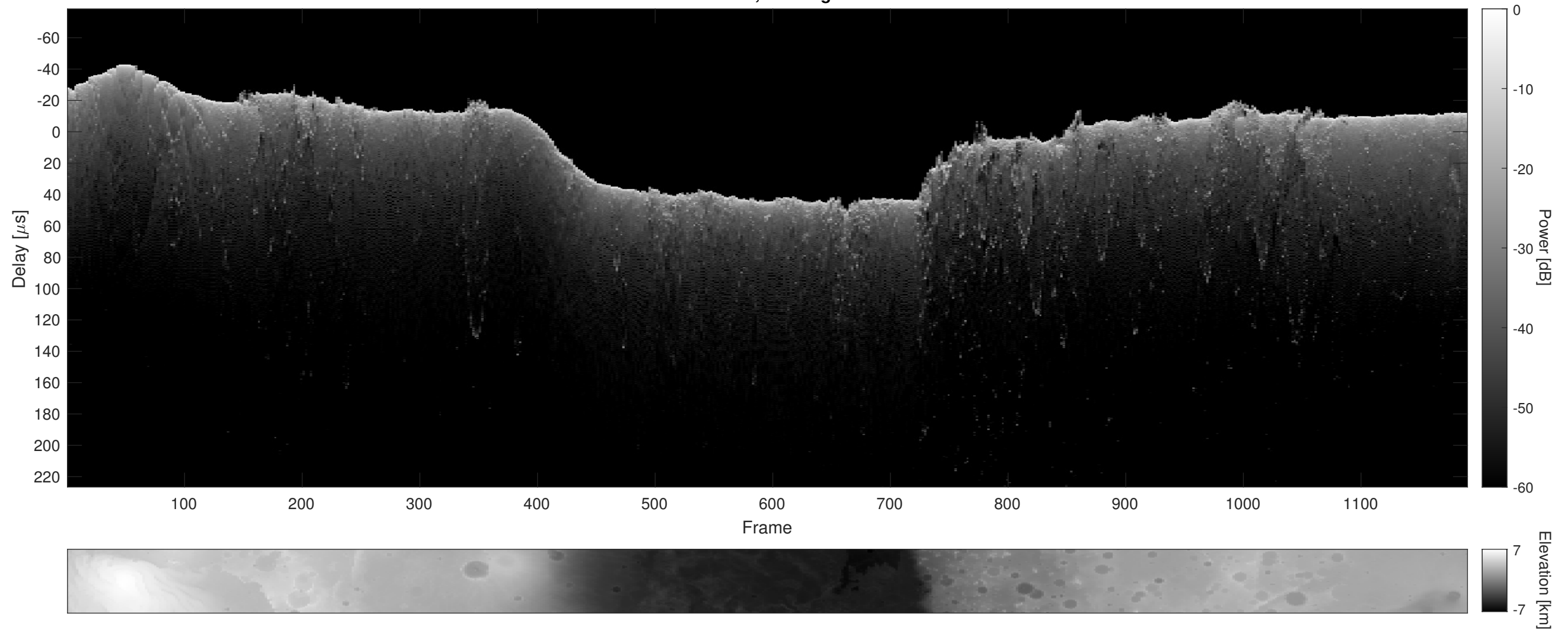
Orbit 8454, Cluttergram
