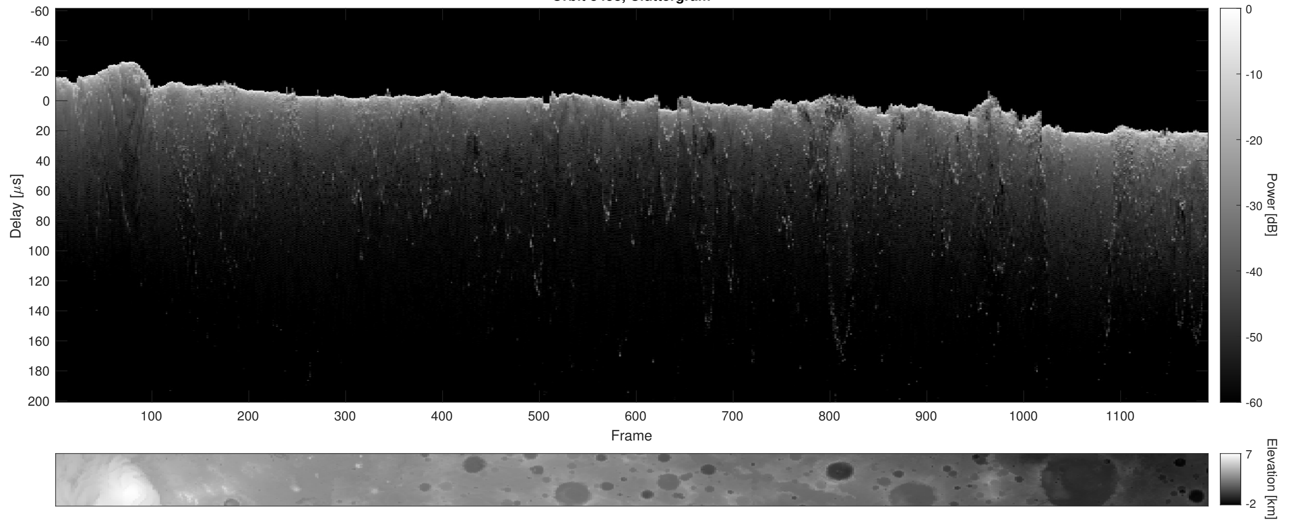
Orbit 8458, Cluttergram
