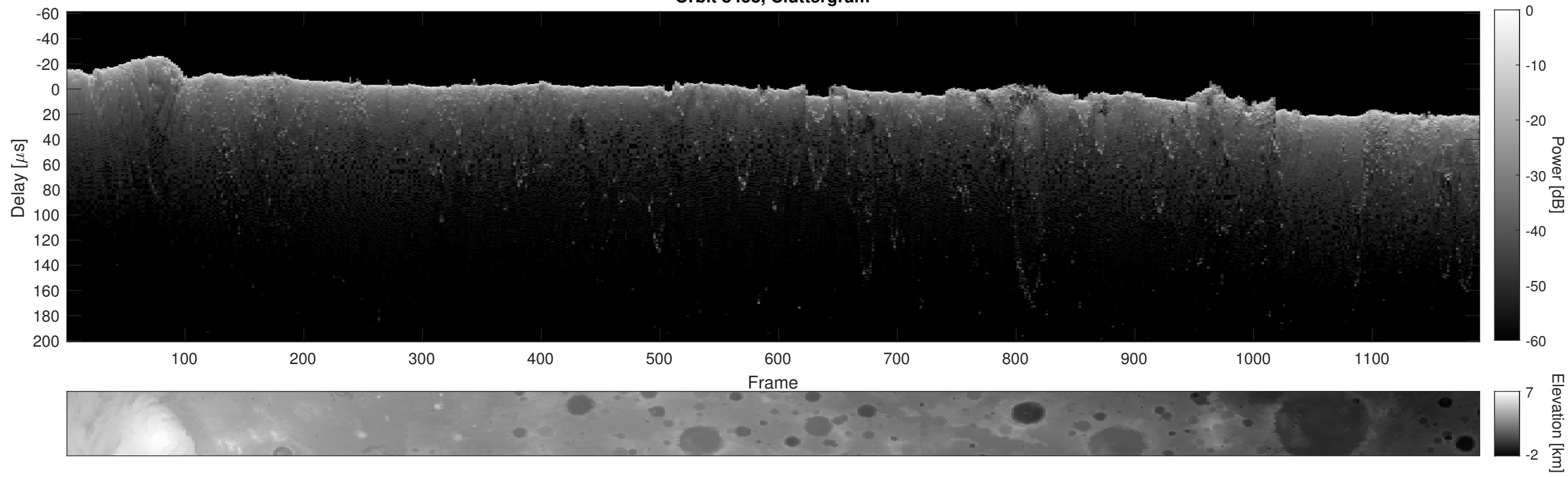
Orbit 8458, Cluttergram
